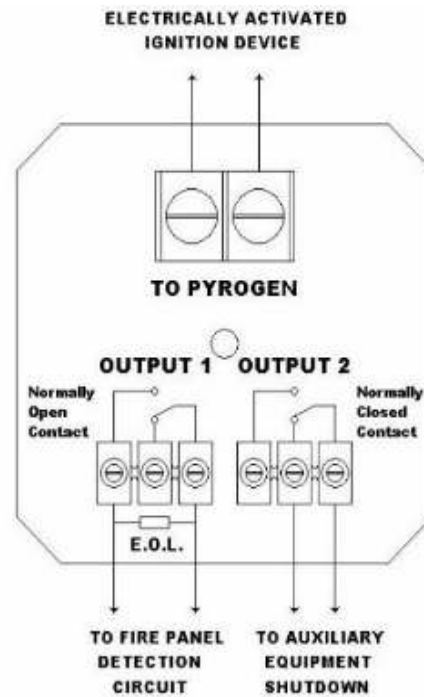
Figure 5: Electrical Connection Diagram (T-Start with Junction Box)
